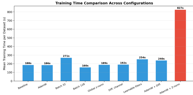
Fig. 4. Training time comparison across multiple configurations demonstrating the runtime trade-offs associated with different batch sizes.
