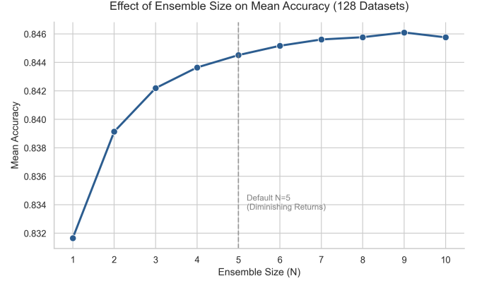
Fig. 6. Effect of ensemble size on classification accuracy. Performance improves with increasing ensemble size before stabilizing.
