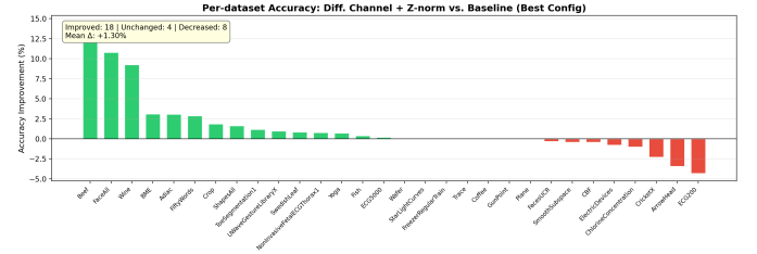
Fig. 2. Dataset-level improvement comparison demonstrating performance gains from optimization strategies including AdamW and differenced input channels.
